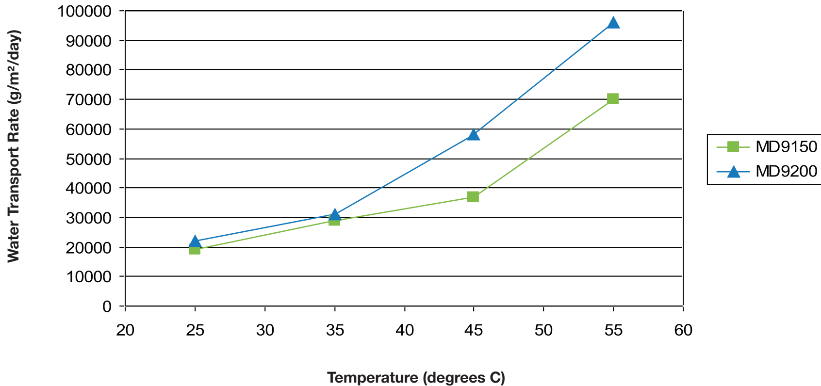
Water Transport vs. Temperature as a Function of Ion Exchange Capacity (IEC) @ 50 % RH
